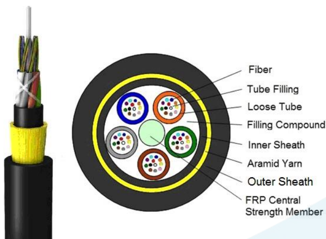
CABLE STRUCTURE AND PARAMETERS:
